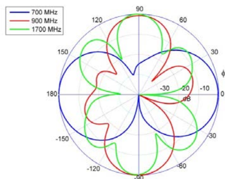
E-Plane (Elevation) – 700, 900, 1700 MHz
